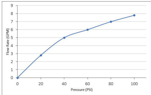
P-2240B Flow Rate (GPM) Vs Pressure (PSI) For Tub Port*
