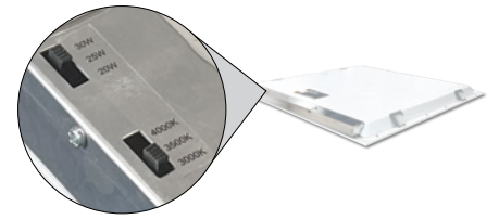
Selectable CCT Three position sliding switch 3000K / 3500K / 4000K
