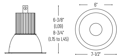
NC2-638 Decorative Glass Reflector (Specify glass separately)
