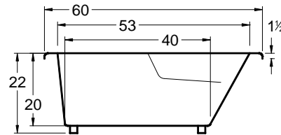
All bathtub dimensions are ± 1/2"
